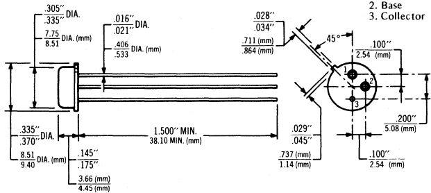
Case TO-5S
