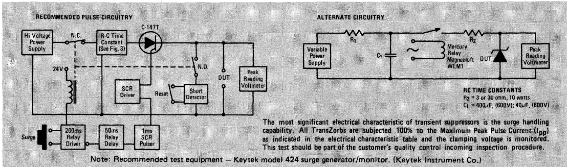
FIGURE 4 - Capacitor Discharge Circuit for Testing TransZorbs
