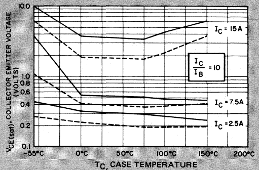
COLLECTOR SATURATION
