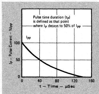
Pulse Wave Form (1.5 x 40 μSec)
