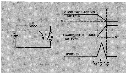
FIGURE 1 — Closing the switch in a resistive circuit creates peak power of 1/4 E_{MAX} I_{MAX} .
