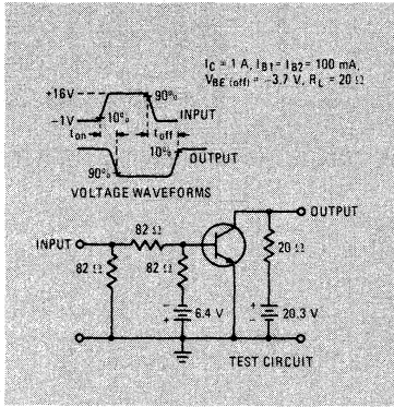
Figure 1 SWITCHING CIRCUIT
