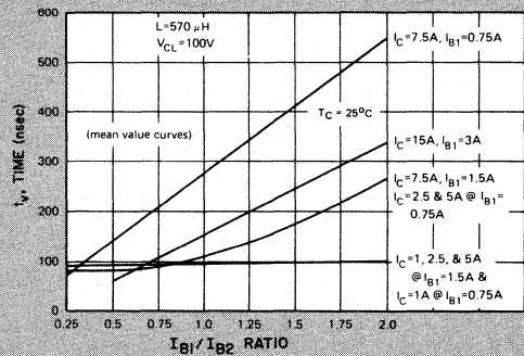
t_v , VOLTAGE RISE TIME vs I_{B1}/I_{B2} RATIO (TURN-OFF, INDUCTIVE)
