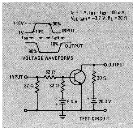
FIGURE 1 — Switching Circuit
