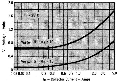
FIGURE 5 — "On" Voltages
