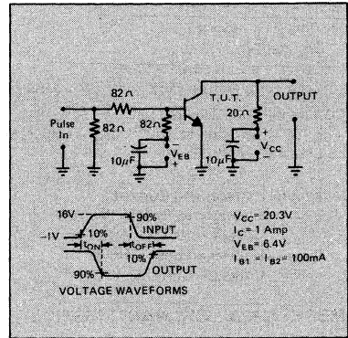
Figure 2 SWITCHING CIRCUIT
