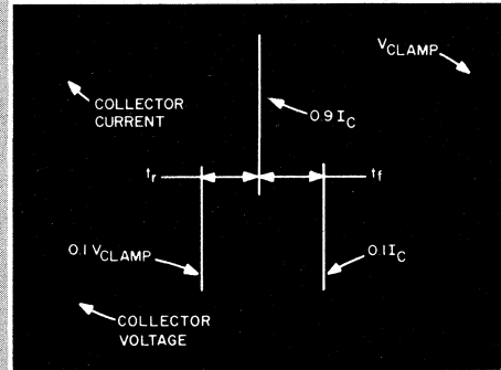
INDUCTIVE SWITCHING TURN-OFF WAVEFORM
