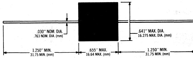
Case 12
