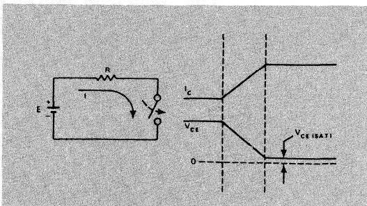
FIGURE 2 — Transistor switching produces the transistor operating conditions depicted here.
