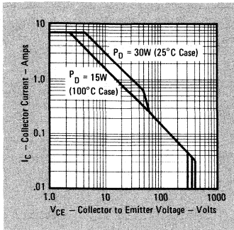
DC Forward Biased Safe Operating Area
