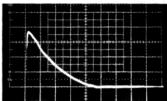
FIGURE 3 - Current Pulse Wave Form Vertical: 50A/cm Horizontal: 20 μsec/cm
