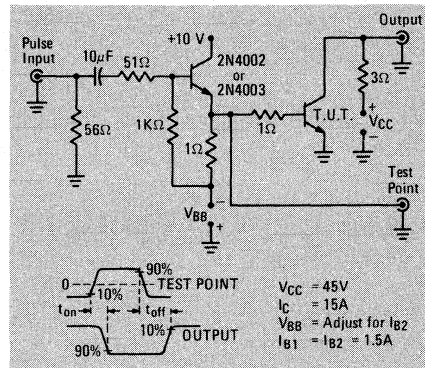
Figure 2 - SWITCHING CIRCUIT
