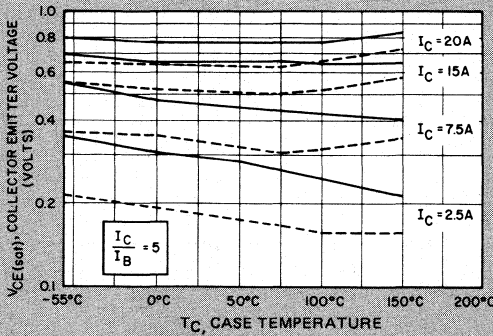
COLLECTOR SATURATION
