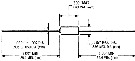
Case DO—7
