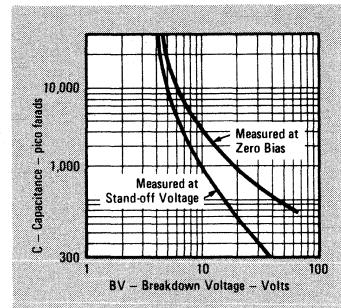
Typical Capacitance vs Breakdown Voltage (Bipolar Types)
