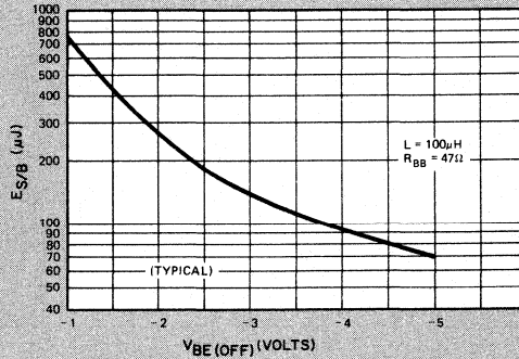
E_S/B CURVE
