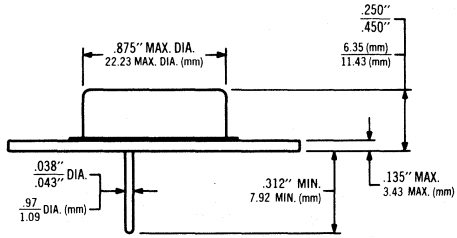
Case TO-3
