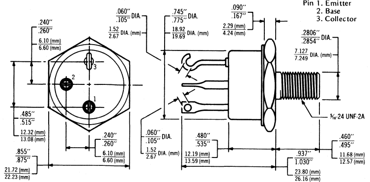
Case TO-63
