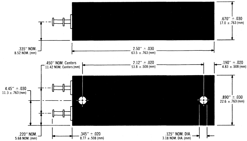
Case 3
