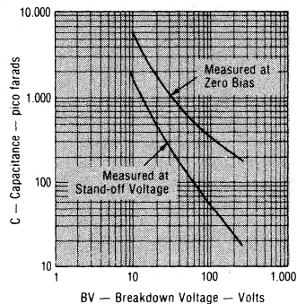
FIGURE 2 Typical Capacitance vs Breakdown Voltage
