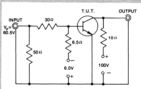
Figure 3— PULSE TEST CIRCUIT
