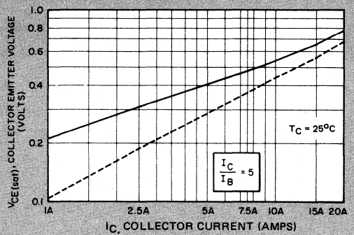
COLLECTOR SATURATION
