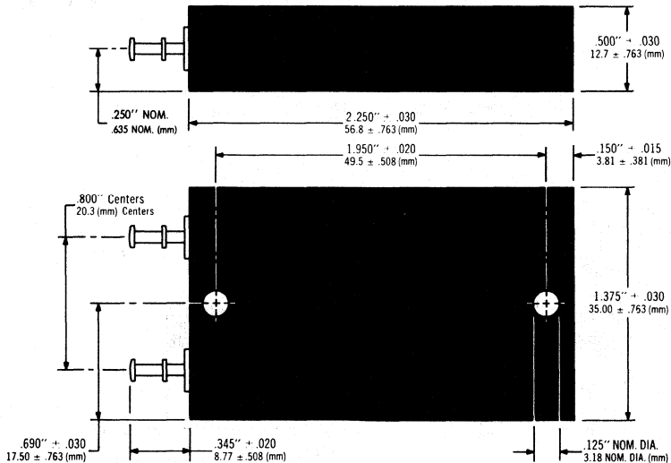
Case 22
