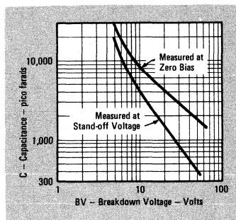
Typical Capacitance vs Breakdown Voltage (Unipolar Types)
