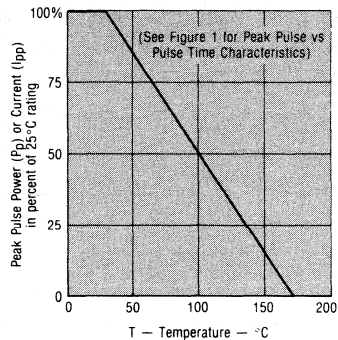
FIGURE 2 — Derating Curve
