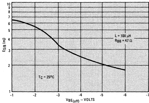
E_{S/B} CURVE
