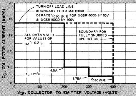
TURN-OFF SAFE OPERATING AREA
