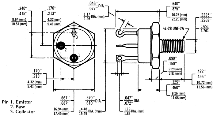
Case TO-63
