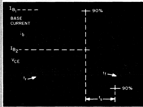
RESISTIVE SWITCHING WAVEFORM
