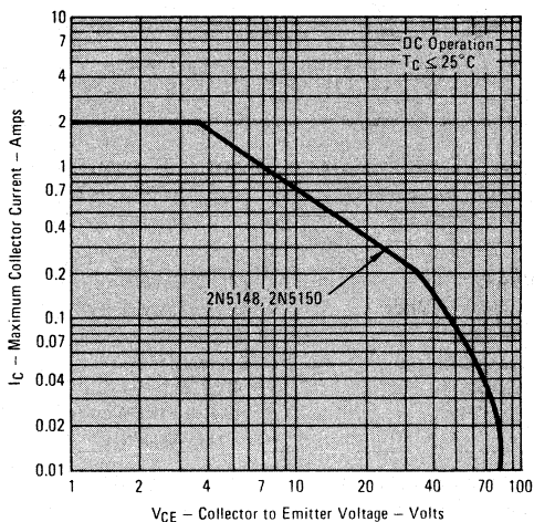
FIGURE 2 — Maximum Safe Operating Region
