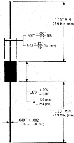
Case 1
