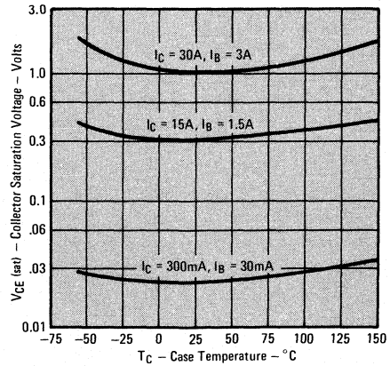
Figure 4 - SATURATION VOLTAGE VS. TEMPERATURE
