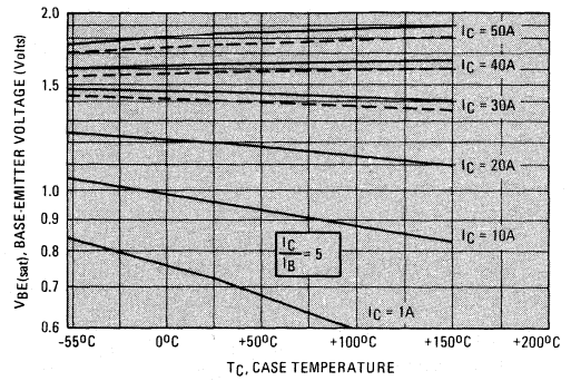
BASE-EMITTER SATURATION
