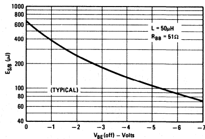
FIGURE 7 - E_s/g Curve
