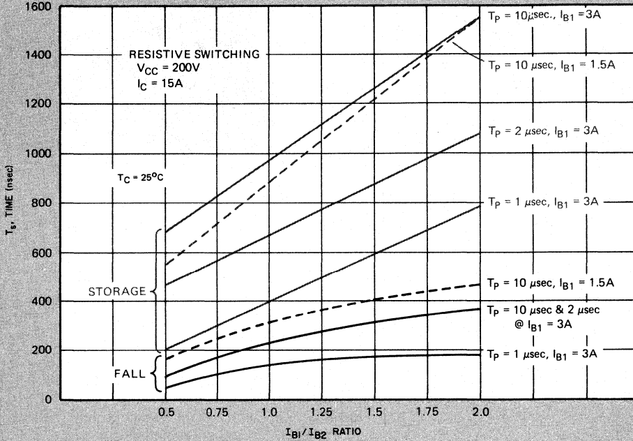
STORAGE & FALL TIME vs PULSE WIDTH ( T_P )
