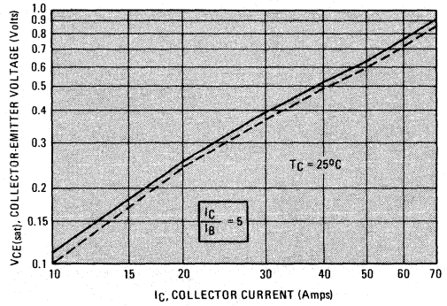
COLLECTOR SATURATION
