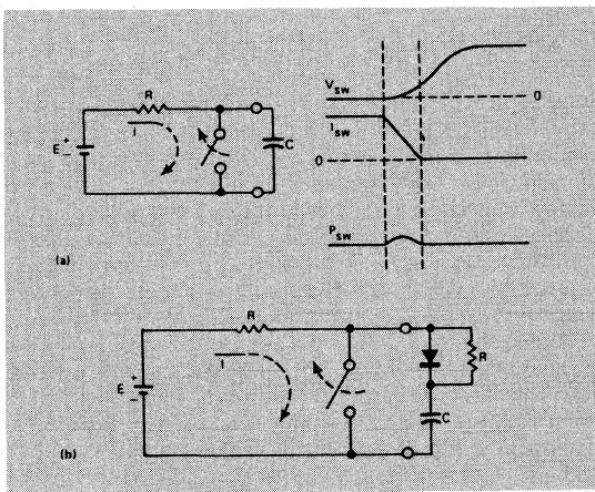
FIGURE 4 — Simple load-line shaping by a capacitor (a) holds back the inductive-circuit voltage rise until current has become low, thereby greatly reducing the peak power. If a diode is added (b), the undesirable retarding of voltage during the switching-ON time is largely avoided.
