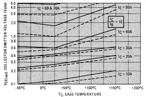
COLLECTOR SATURATION
