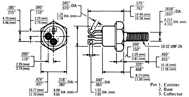
Case TO-59
