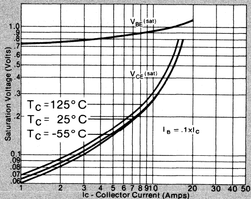
Figure 2— TYPICAL SATURATION VOLTAGE
