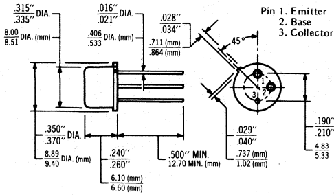
Case TO-39
