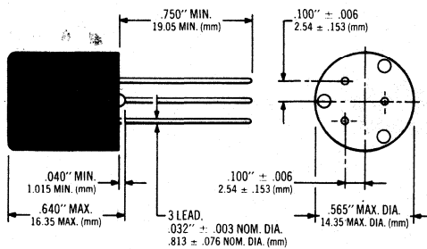
Case 10
