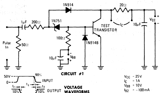
PULSE RESPONSE MEASUREMENT CIRCUIT
